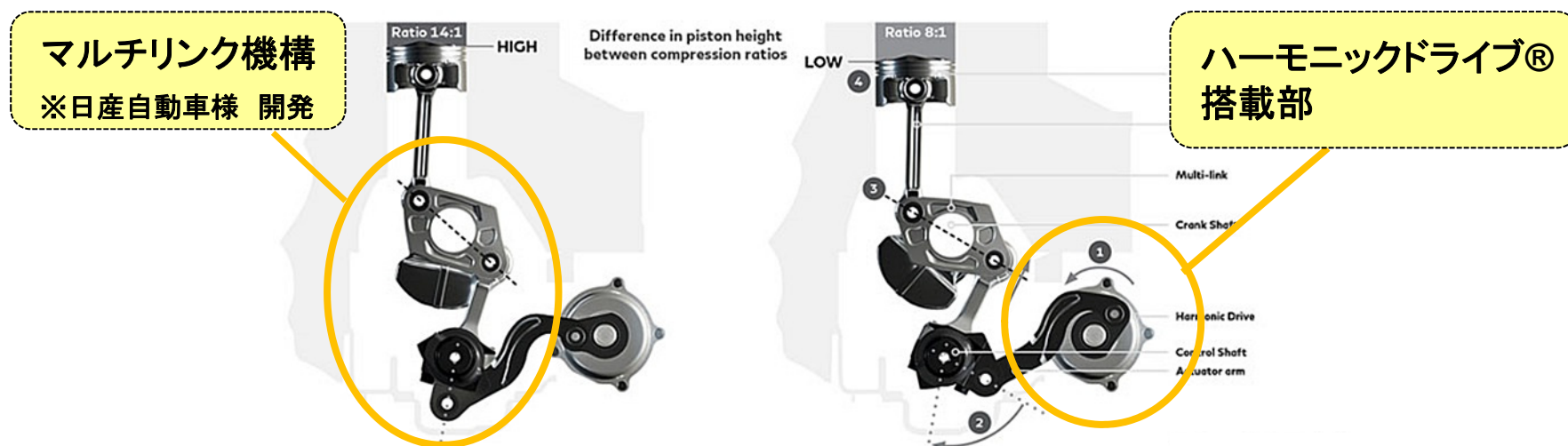
COMPARISON OF VC-T TECHNOLOGY IN HIGH AND LOW COMPRESSION RATIOS
